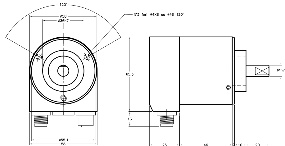
MEM540Bus
